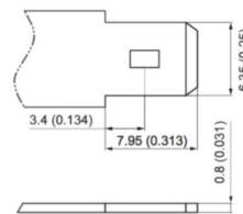
F2 Terminal Unit: mm (inches)
